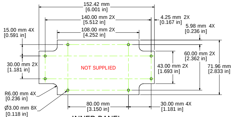
INNER PANEL
