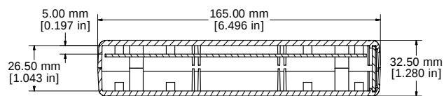
SECTION B-B
