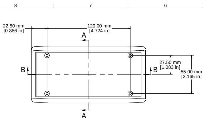
ASSEMBLY - TOP
