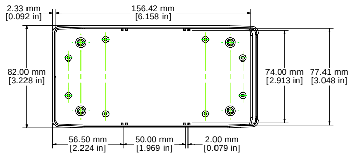
BOX - INSIDE
