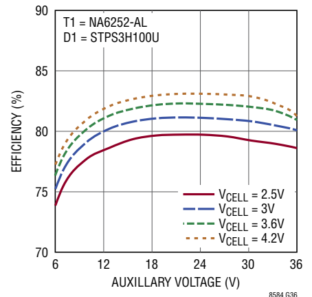
Conversion Efficiency
