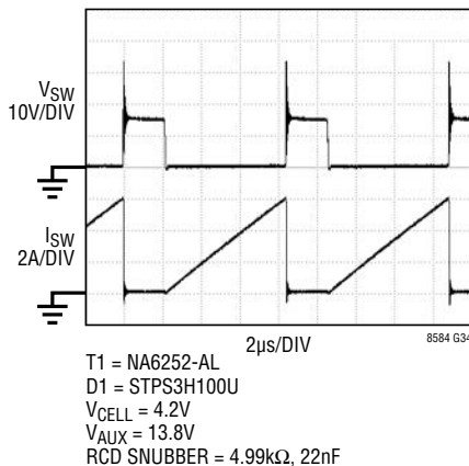
Switching Waveform
