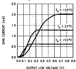
LP2951 Comparator Sink Current
