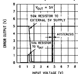
LP2951 Error Comparator Output
