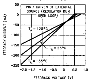
LP2951 Feedback Pin Current
