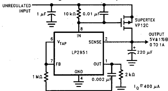
1A Regulator with 1.2V Dropout
