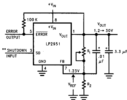
FIGURE 2. Adjustable Regulator
