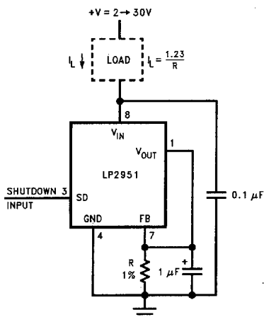
Low Drift Current Source
