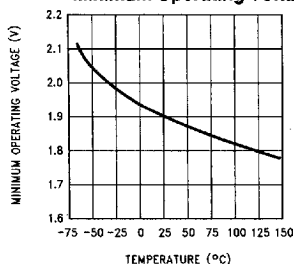
LP2951 Minimum Operating Voltage
