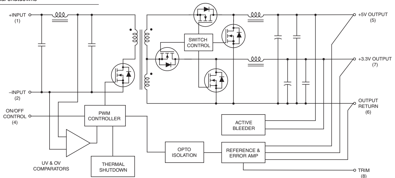
Figure 1. Simplified Schematic
