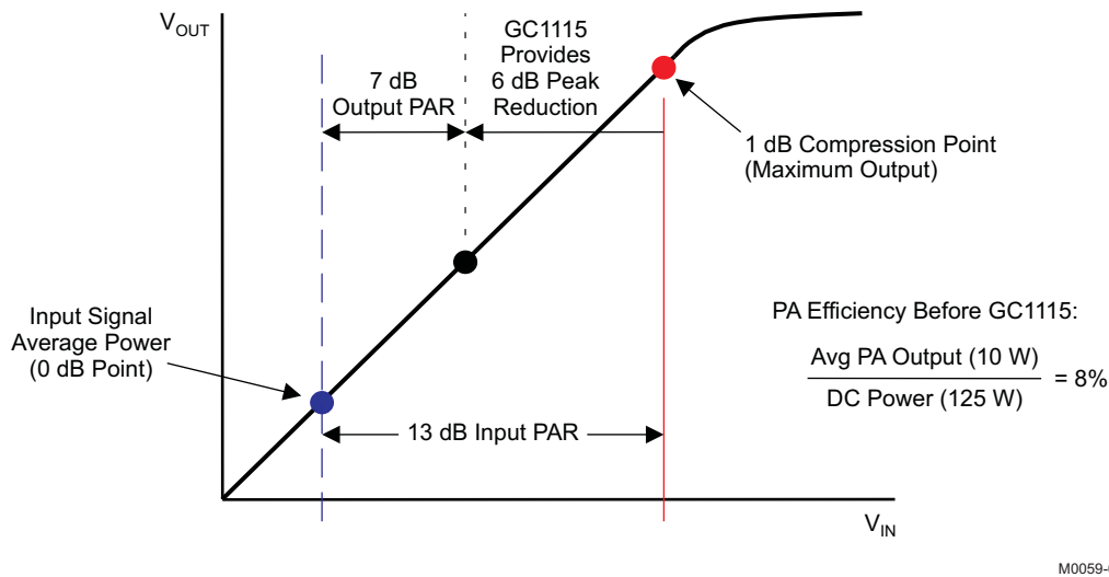
Figure 2. Reducing the Peak-to-Average Ratio (PAR)
