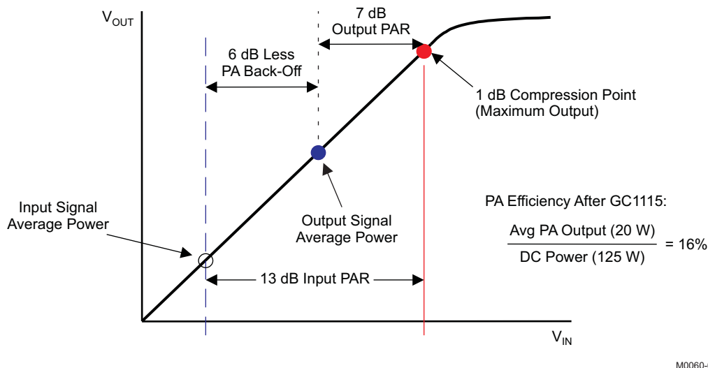
Figure 3. Increasing PA Efficiency
