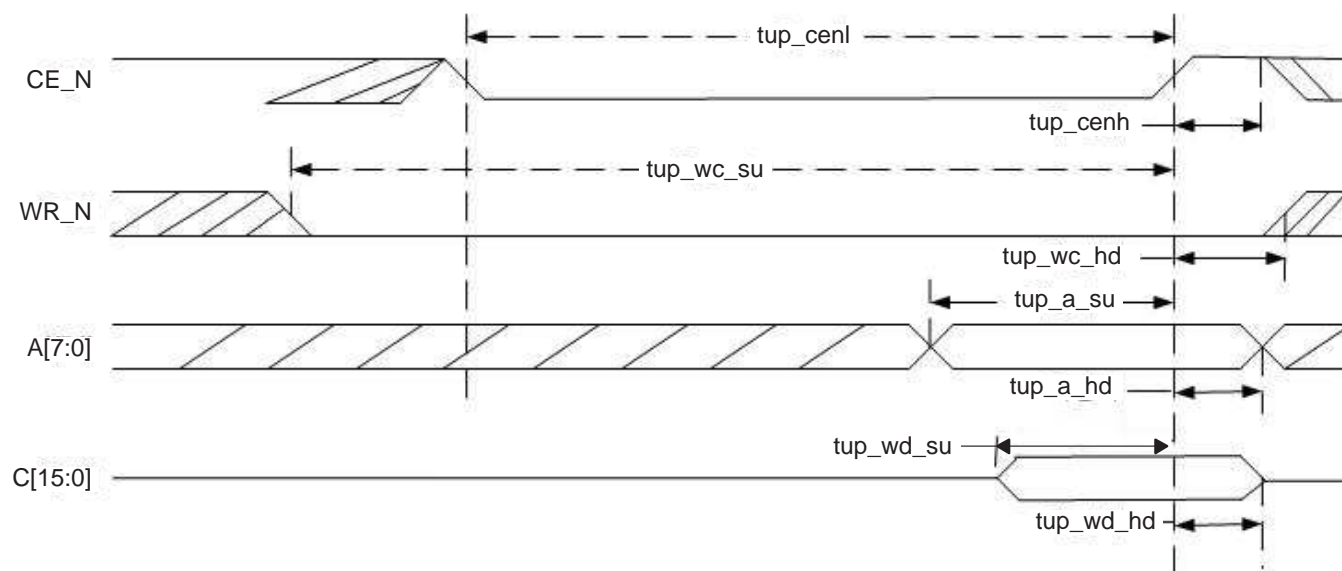
Figure 17. Write Cycle – \overline{RD} Held Low
