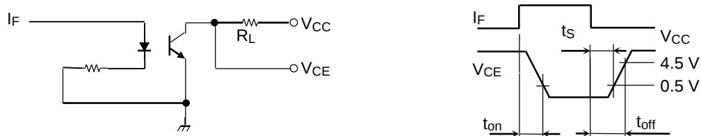
Figure 1: Switching Time Test Circuit
