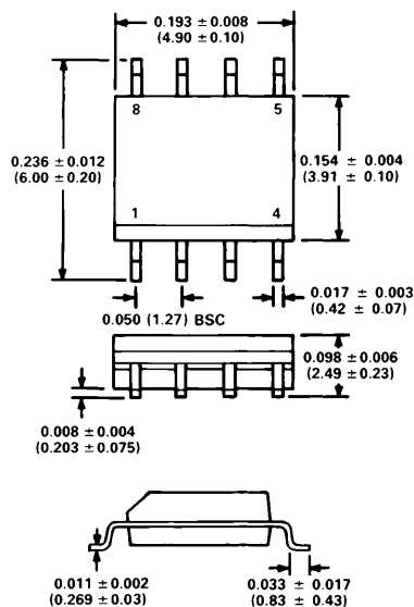
8-Pin SOIC (R) Package
