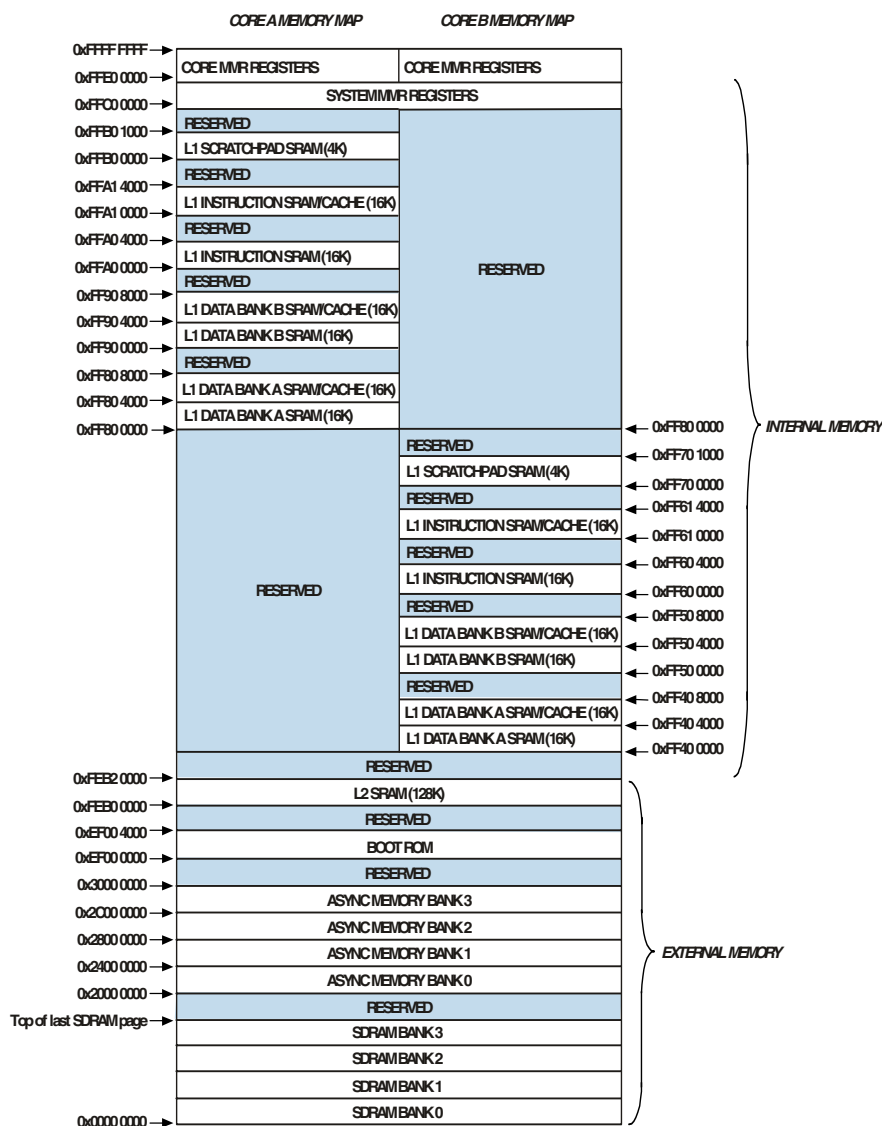
Figure 3. Memory Map
