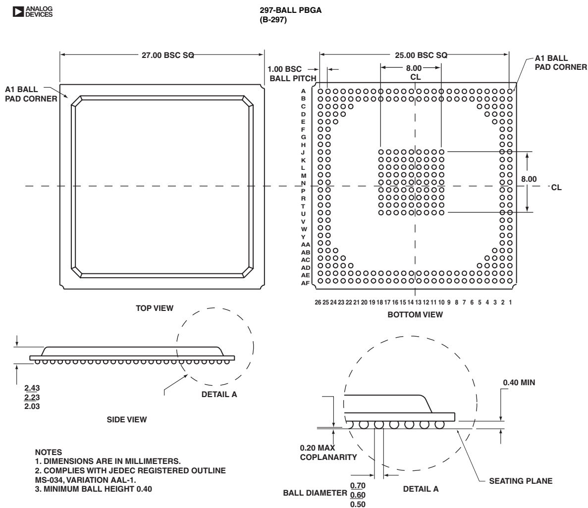
Figure 30. 297-Ball PBGA Grid Array
