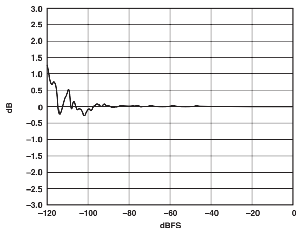
TPC 4. Linearity Plot
