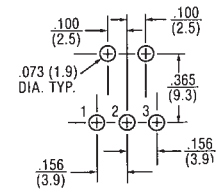
Mounting Information
