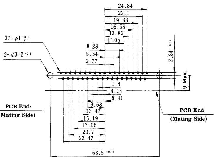
RDGD-37
