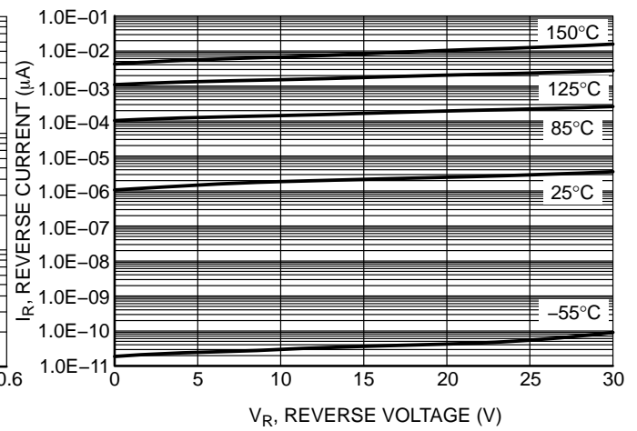
Figure 2. Reverse Leakage
