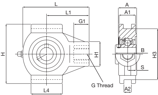
PST SERIES
