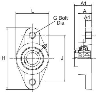
PSFT SERIES
