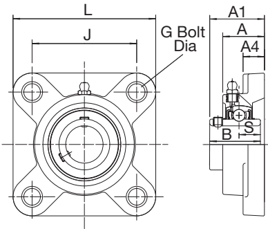
PSF SERIES
