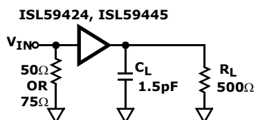
FIGURE 18A. TEST CIRCUIT WITH OPTIMAL OUTPUT LOAD
