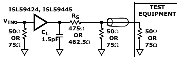
FIGURE 18B. TEST CIRCUIT FOR MEASURING WITH 50Ω OR 75Ω INPUT TERMINATED EQUIPMENT
