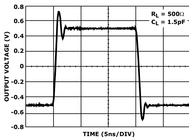
FIGURE 6. ISL59445 TRANSIENT RESPONSE
