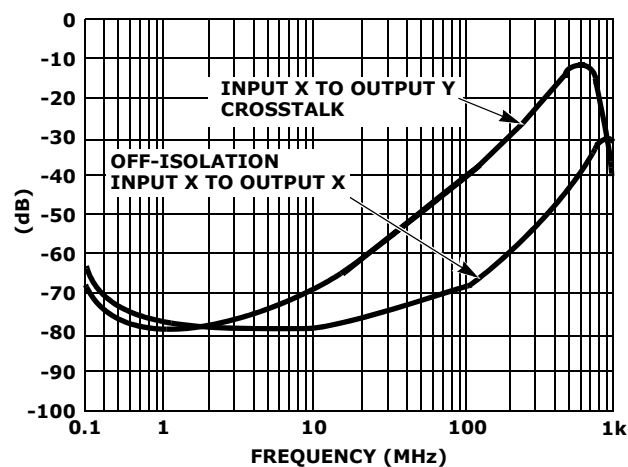
FIGURE 8. ISL59445 CROSSTALK AND OFF-ISOLATION
