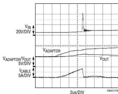
FIGURE 5 CIRCUIT R_{IN} = 150\mu\Omega , L_{IN} = 2\mu H LOAD = 10\Omega , C_{OUT} = 10\mu F
