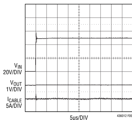
FDC5612 R_{IN} = 150m\Omega , L_{IN} = 0.7\mu H LOAD = 10\Omega , C_{OUT} = 10\mu F
