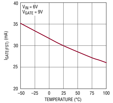
GATE Fast Pull-Down Current vs Temperature
