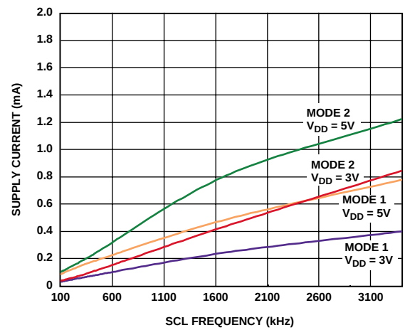
Figure 15. AD7994 Average Supply Current vs. I^2\text{C} Bus Rate for V_{DD} = 3\text{ V} and 5\text{ V}
