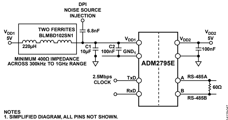
Figure 50. Typical Setup for DPI IEC 62132-4 Noise Immunity Test
