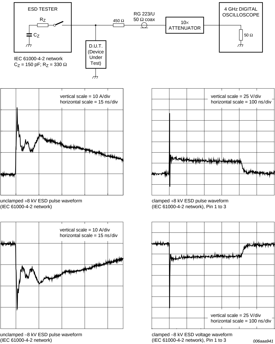
Fig 9. ESD clamping test setup and waveforms
