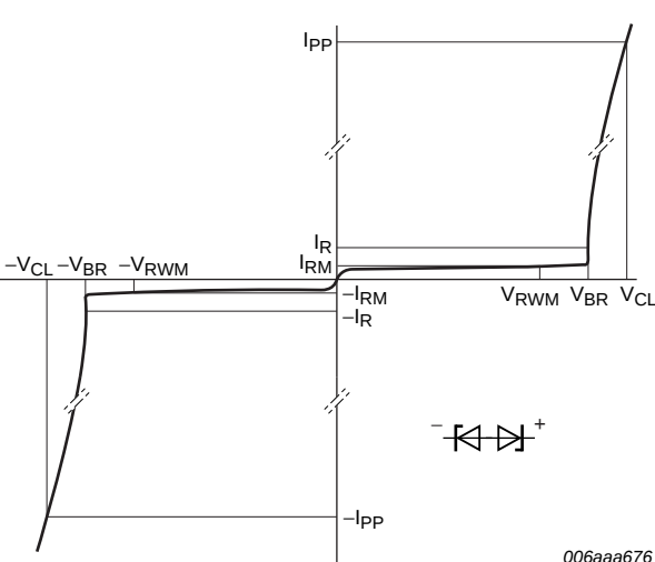
Fig 6. Reverse current as a function of reverse voltage; typical values
