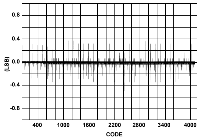
FIGURE 7. TYPICAL DNL
