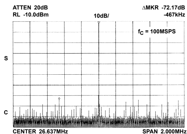
FIGURE 17. SPURIOUS FREE DYNAMIC RANGE = 72.17dBc
