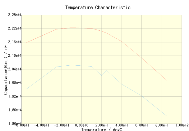
C3225X5R0J226M200AA(DC Bias = 0V) C3225X5R0J226M200AA(DC Bias = 3.15V)
