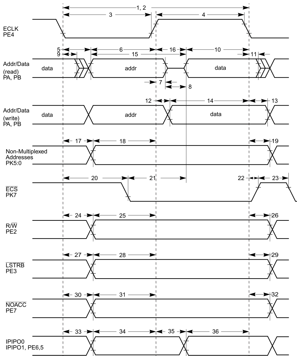
Figure A-9. General External Bus Timing
