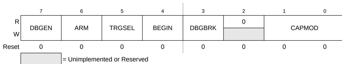
Figure 16-4. Debug Control Register (DBGCR1)
