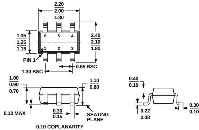
Figure 46. 6-Lead Thin Shrink Small Outline Transistor Package [SC70] (KS-6)
