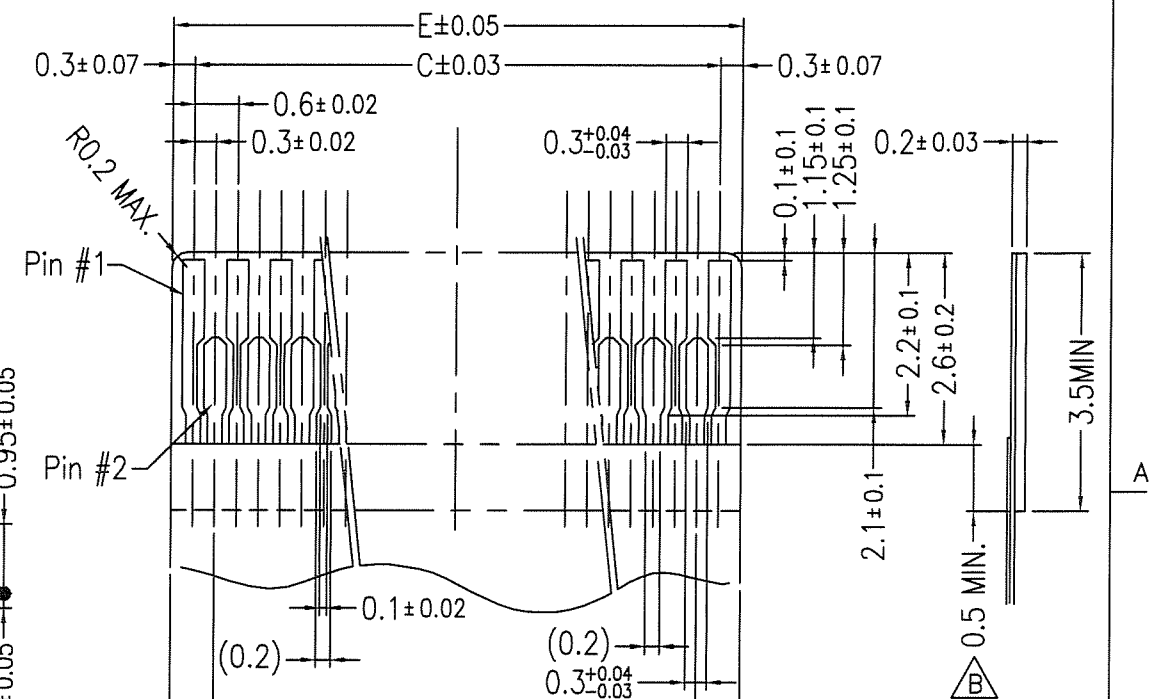
RECOMMENDED FPC CONFIGURATION
