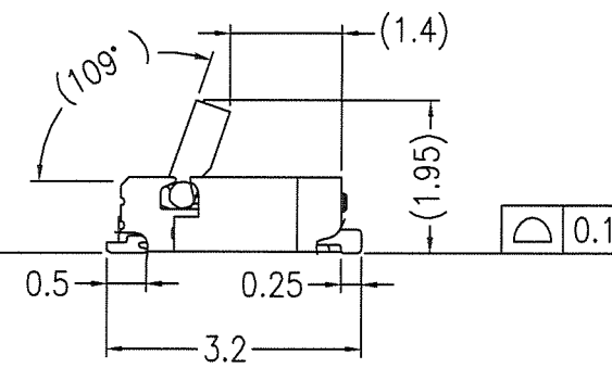
ACTUATOR OPEN CONDITION
