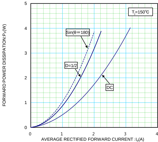
I_O - P_F CHARACTERISTICS
