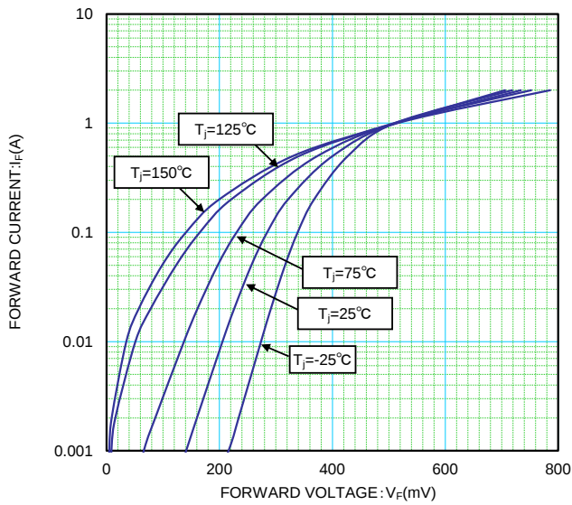
V_F - I_F CHARACTERISTICS
