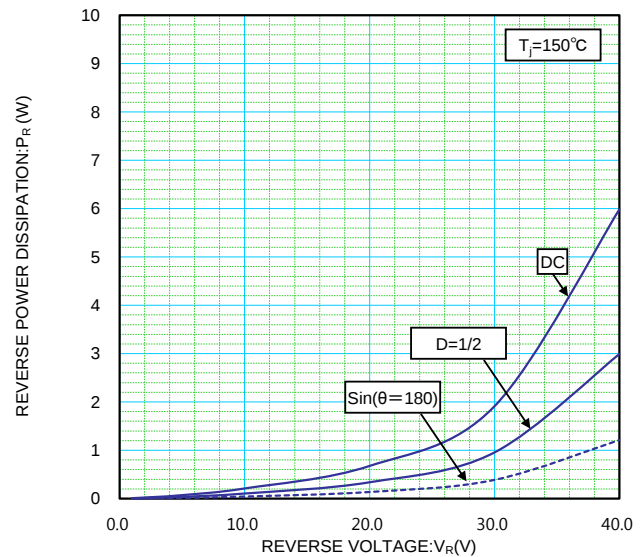
V_R - P_R CHARACTERISTICS
