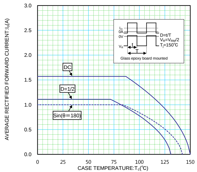
DERATING CURVE ( I_O - T_c )
