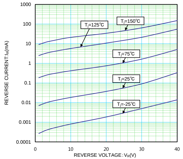
V_R - I_R CHARACTERISTICS
