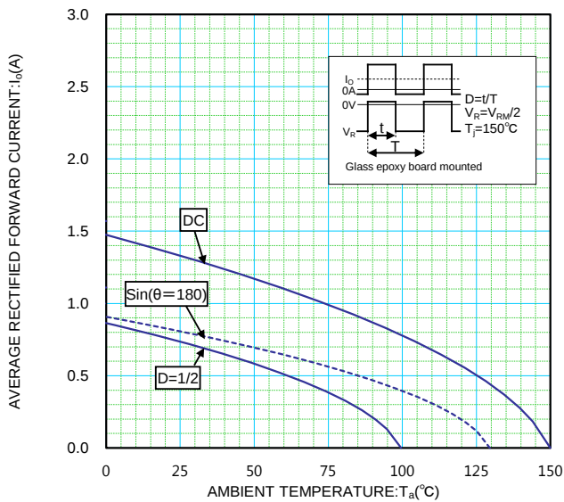
DERATING CURVE ( I_O - T_a )
