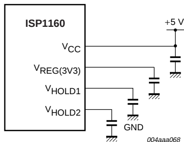
Fig 29. Using a 5 V supply.
