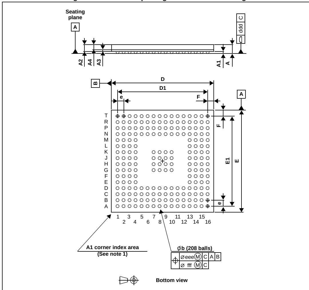
Figure 37. LBG208 package mechanical drawing
