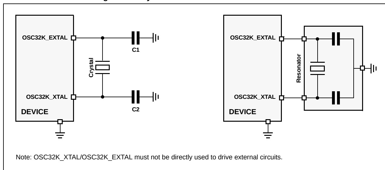
Figure 15. Crystal oscillator and resonator connection scheme
