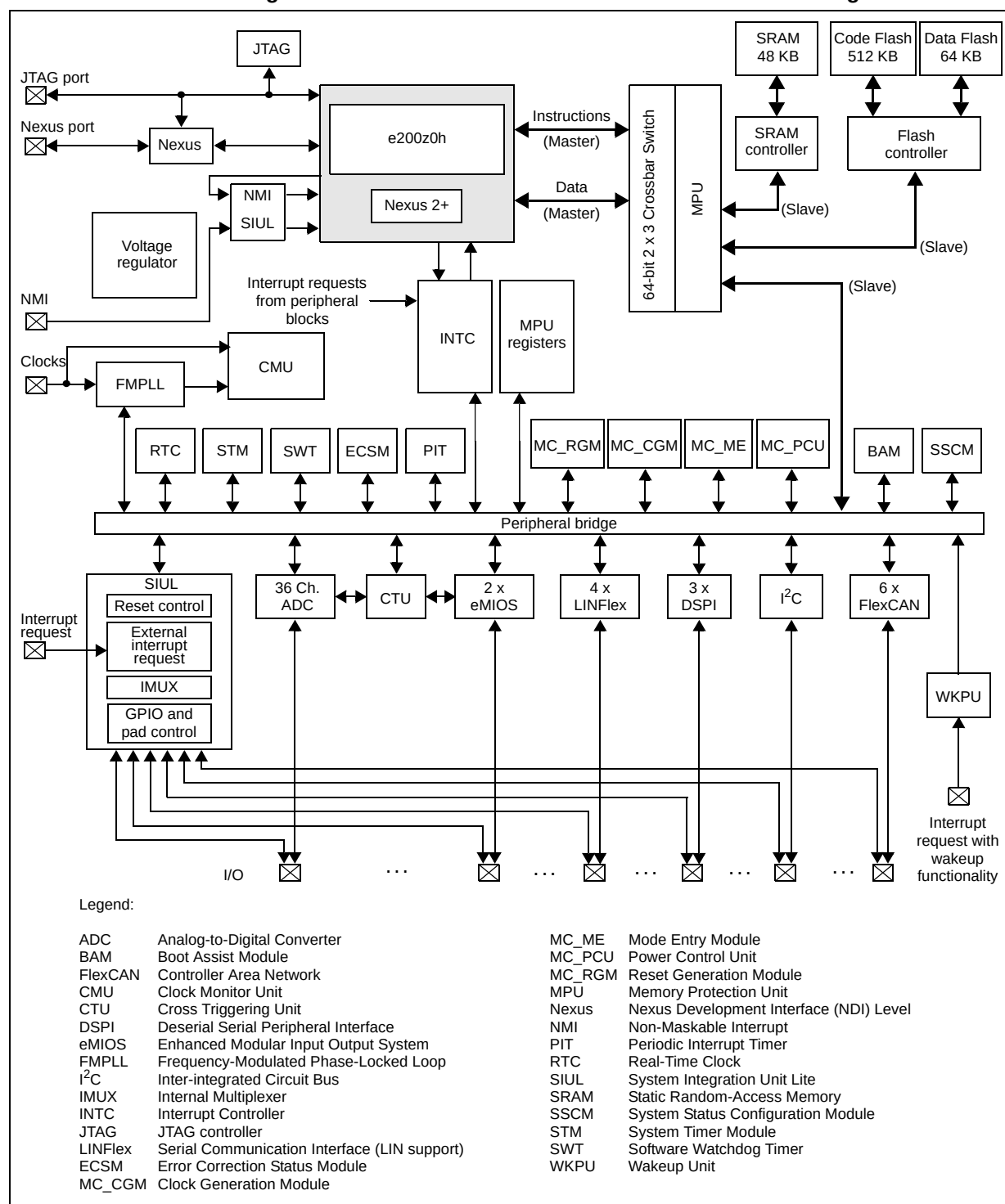
Figure 1. SPC560B40x/50x and SPC560C40x/50x block diagram
