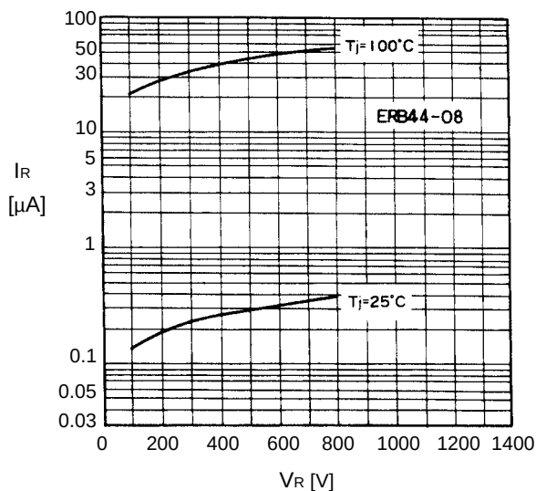
Reverse characteristics
