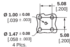
Recommended Mounting Holes
