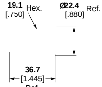
N Series Jack – 7 mm Plug
