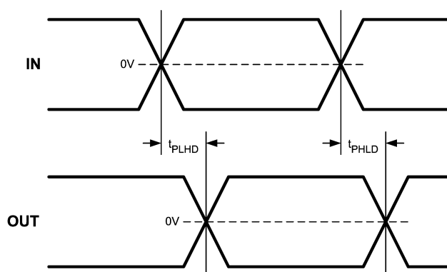
Figure 4. Propagation Delay Timing Diagram
