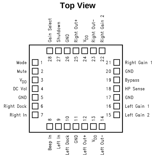
Figure 2. WQFN Package See Package Number NJB0028A for Exposed-DAP WQFN
