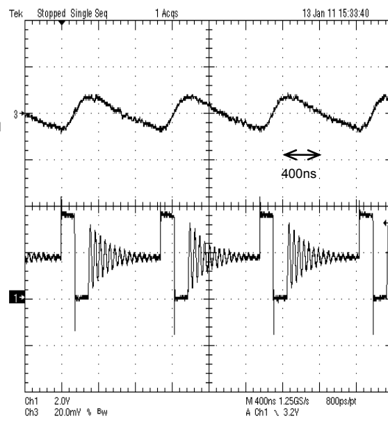
Figure 10. PFM mode Operation, I_{out}=50\text{mA}
