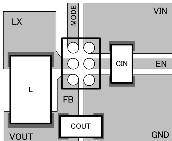
Figure 19. PCB layout
