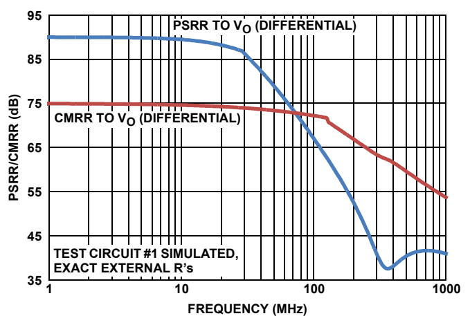
FIGURE 25. PSRR/CMRR TO DIFFERENTIAL V_O
