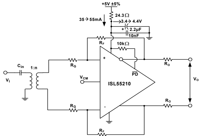
FIGURE 32. OPERATING FROM A SINGLE +5V SUPPLY
