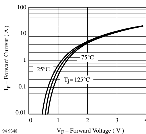
Figure 3. Typ. Forward Current vs. Forward Voltage
