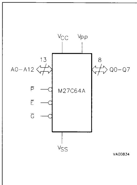
Figure 1. Logic Diagram
