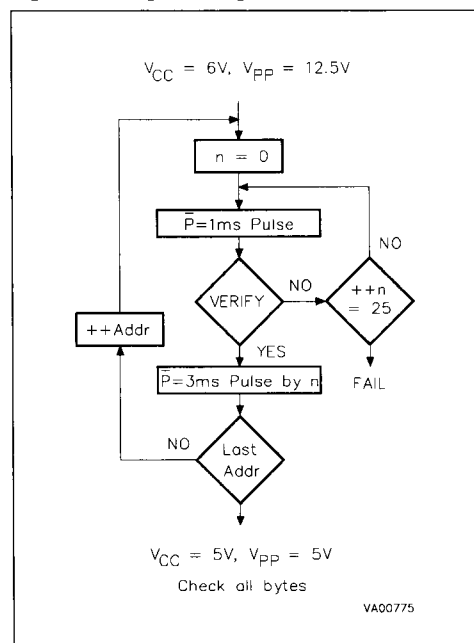
Figure 7. Programming Flowchart
