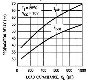
MM78C29/MM88C29 Typical Propagation Delay vs Load Capacitance
