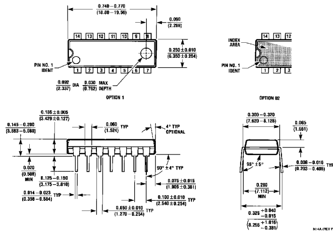
Molded Dual-In-Line Package (N) Order Number MM78C29N, MM78C30N, MM88C29N or MM88C30N NS Package Number N14A
