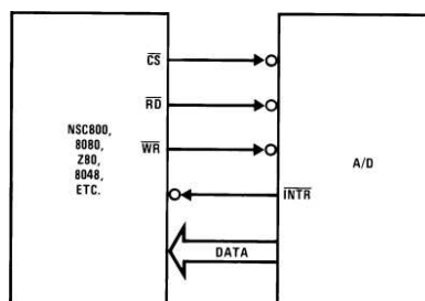
8080 Interface
