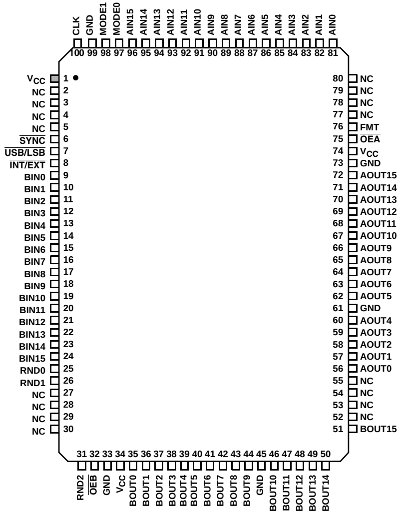
HSP43216JC (100 LD MQFP) TOP VIEW
