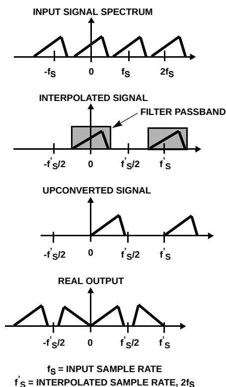
FIGURE 18. QUADRATURE TO REAL CONVERSION
