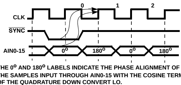
FIGURE 17. DATA SYNCHRONIZATION WITH PHASE OF DOWN CONVERT LO
