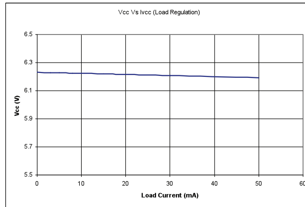
Figure 7. VCC Load Regulation
