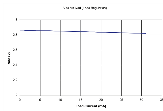
Figure 8. VDD Load Regulation
