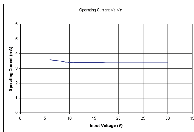
Figure 6. Operating Current Vs VIN
