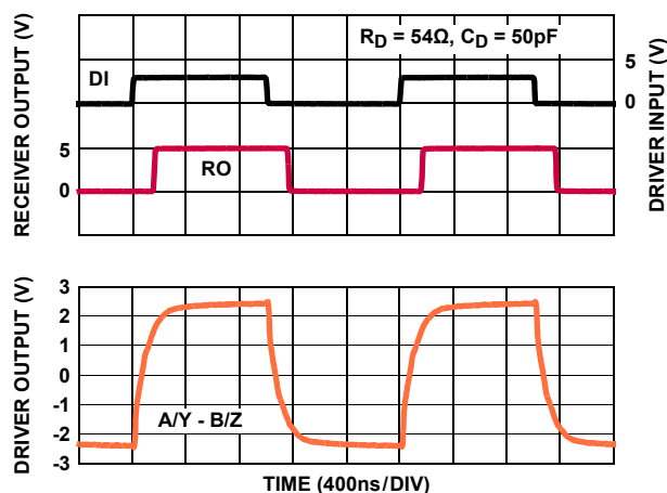
FIGURE 26. DRIVER AND RECEIVER WAVEFORMS (ISL32475E)
