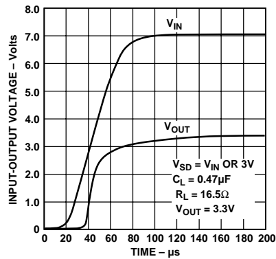
Figure 10. Power-Up Transient
