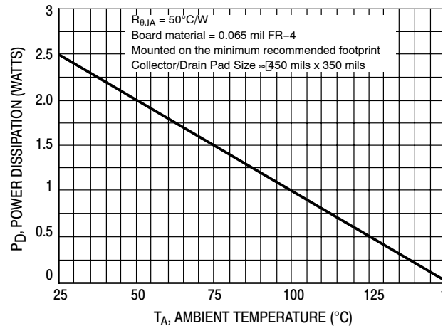
Figure 15. D 2 PAK Power Derating Curve
