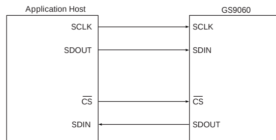
Figure 3-8: Gennum Serial Peripheral Interface (GSPI)
