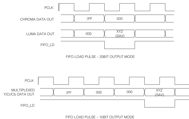
Figure 3-5: \overline{\text{FIFO\_LD}} Pulse Timing
