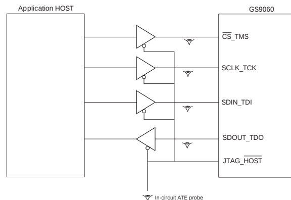
Figure 3-13: In-Circuit JTAG
