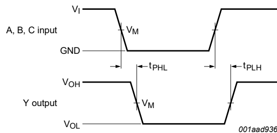
Fig. 4. The input A, B and C to output Y propagation delays
