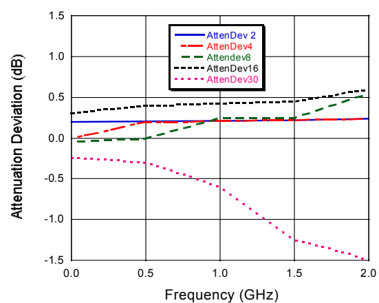
Attenuation Accuracy
