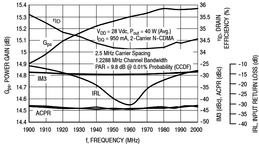
Figure 4. 2-Carrier N-CDMA Broadband Performance @ P_{out} = 40 Watts Avg.
