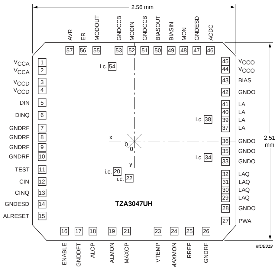
Fig.10 TZA3047UH die.
