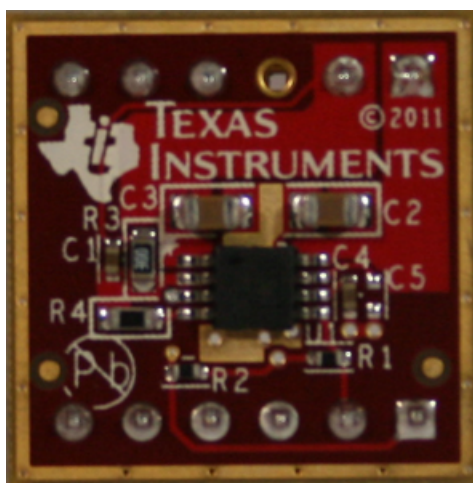
Figure 1. SMP-TPS7A4901-MVK Submodule
