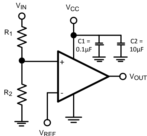
Figure 1. Threshold Detector
