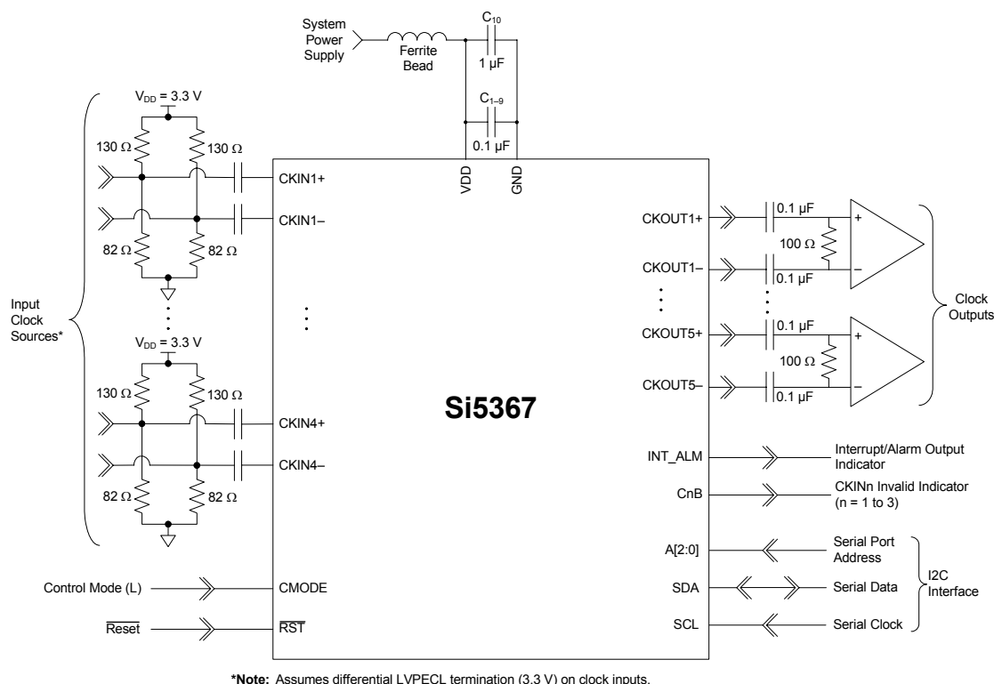
Figure 2. Si5367 Typical Application Circuit (I 2 C Control Mode)
