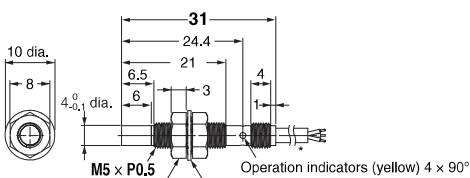
Operation indicators (yellow) 4 x 90° M5 x P0.5 Two clamping nuts Toothed washer * 2.9-dia. vinyl-insulated round cable with 3 conductors (Conductor cross section: 0.14 mm², Insulator diameter: 0.8 mm), Standard length: 2 m Model with robot (bending-resistant) cable: 2.9-dia. vinyl-insulated round cable with 3 conductors (Conductor cross section: 0.15 mm², Insulator diameter: 1.05 mm), Standard length: 2 m
