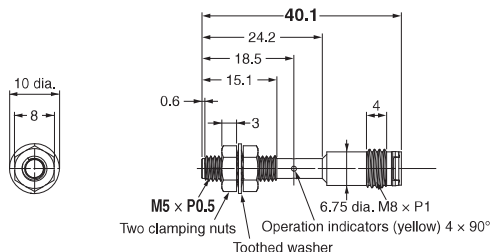
Operation indicators (yellow) 4 x 90° M8 x P1
