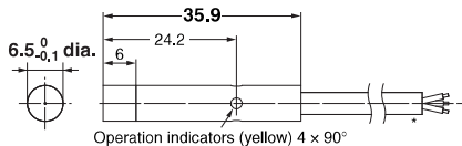
Operation indicators (yellow) 4 x 90° * 4-dia. vinyl-insulated round cable with 3 conductors (Conductor cross section: 0.14 mm², Insulator diameter: 0.85 mm), Standard length: 2 m Model with robot (bending-resistant) cable: 4-dia. vinyl-insulated round cable with 3 conductors (Conductor cross section: 0.3 mm², Insulator diameter: 1.2 mm), Standard length: 2 m
