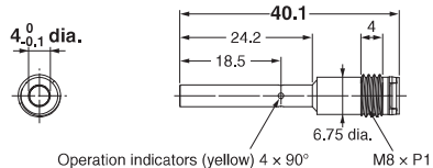
Operation indicators (yellow) 4 x 90° M8 x P1
