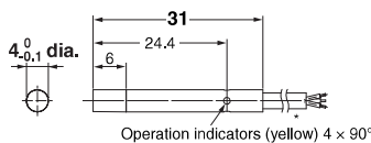
Operation indicators (yellow) 4 x 90° * 2.9-dia. vinyl-insulated round cable with 3 conductors (Conductor cross section: 0.14 mm², Insulator diameter: 0.8 mm), Standard length: 2 m Model with robot (bending-resistant) cable: 2.9-dia. vinyl-insulated round cable with 3 conductors (Conductor cross section: 0.15 mm², Insulator diameter: 1.05 mm), Standard length: 2 m
